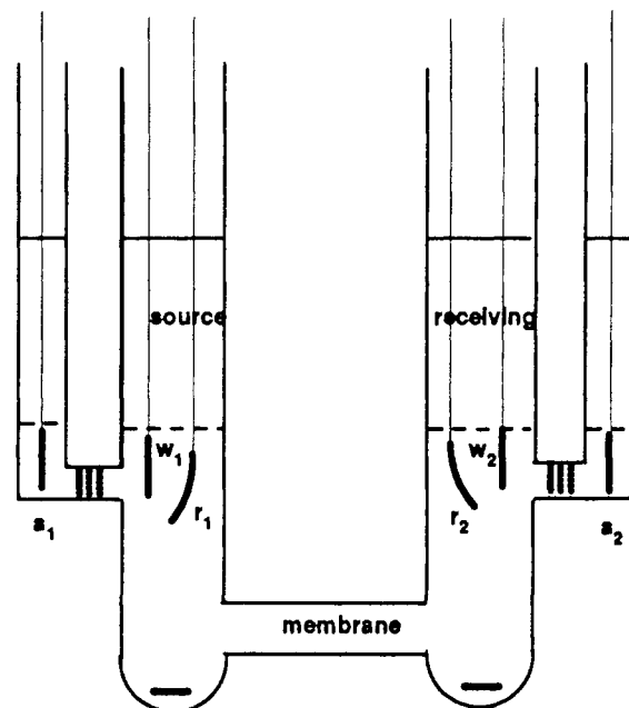
Figure 1. Diagram of transport cell showing the two 3-Pt-electrode configurations ( a_1 , w_1 , r_1 , for reduction and a_2 , w_2 , r_2 for oxidation) source phase = 0.1–1.0 M MClO_4 in H_2O ; receiving phase = distilled, deionized water; membrane phase = 0.5–2.0 mM ligand and 0.1 M TBAP in CH_2Cl_2 . Note that auxiliary electrodes are separated from their corresponding working electrodes and reference electrodes by fine porosity glass filters.
